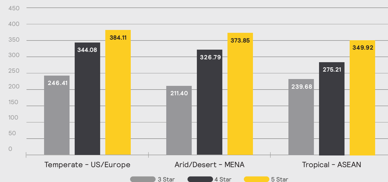
Figure 1 – Average energy use intensity (EUI) by region for different hotel types (kWh/m 2 .yr)
