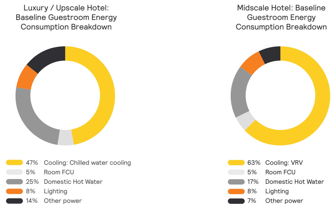
Figure 3: Baseline hotel guest room energy in Singapore
