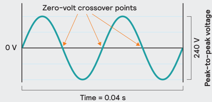
Example of ideal power supply
