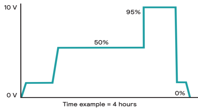
Lighting control system varies between 0-10 V to adjust the output level.
